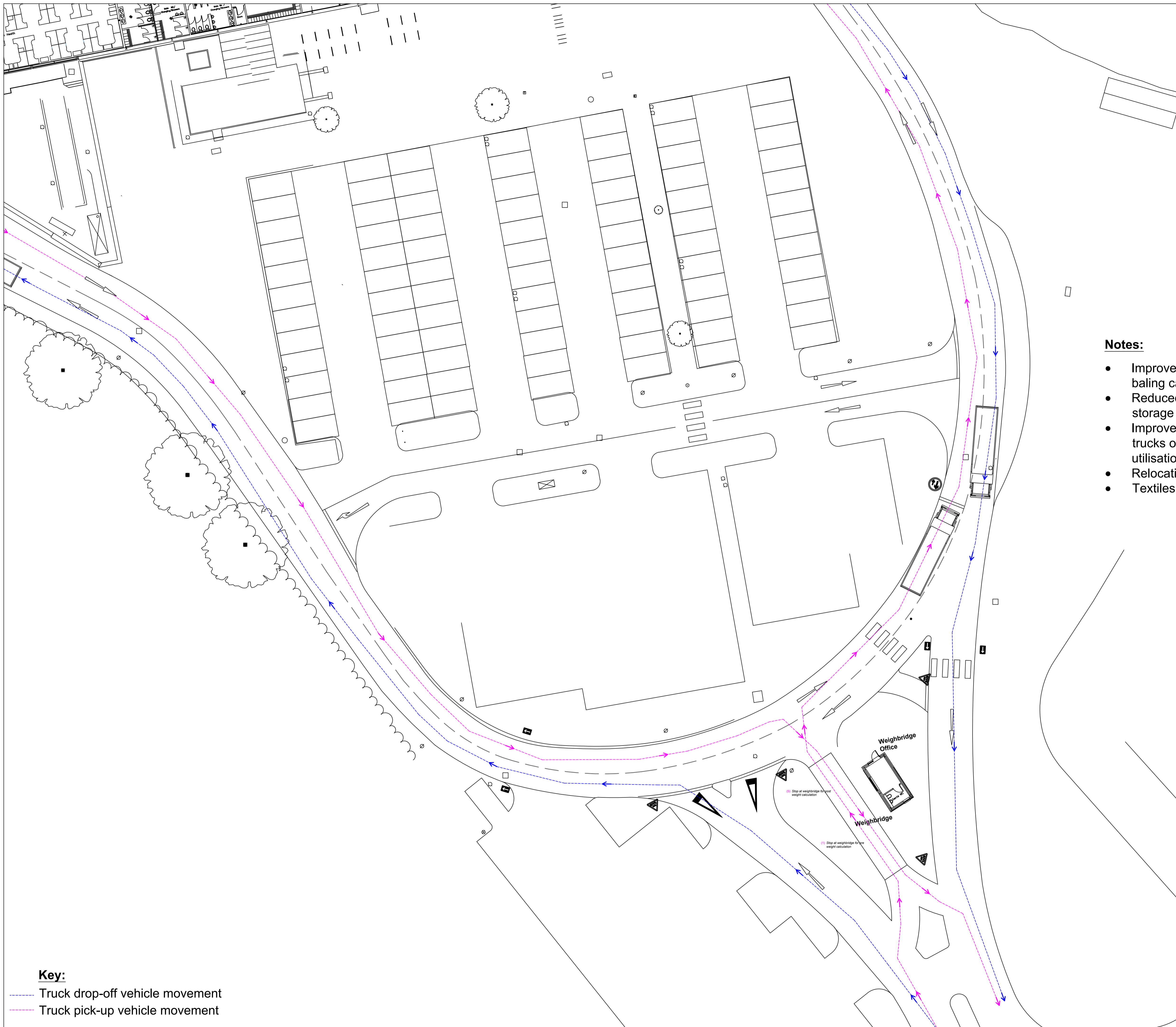
Site Plan
